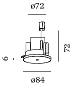
BH | SEMI RECESSED SINGLE BASE
