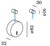
IH | WALL BASE for 1 luminaire | incl. 2 wall-ceiling brackets | for cable 4.25-5.5mm diameter | incl. switch on/off
